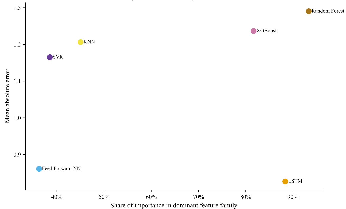
Accuracy vs Feature Family Concentration
